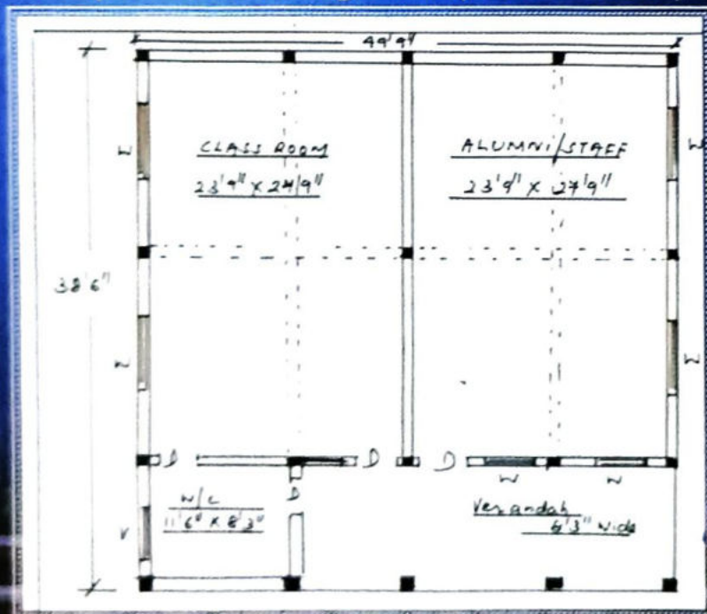
Proposed Building Plan (I and II Floor)
